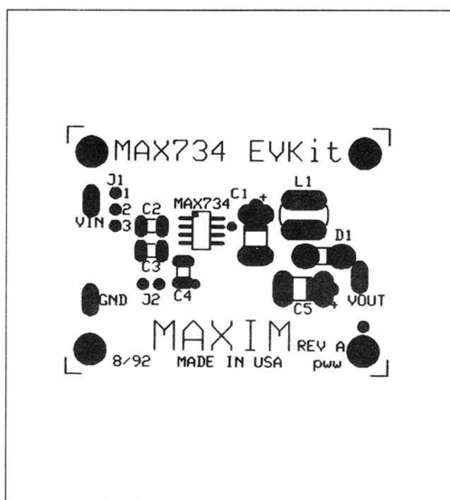
Figure 5. Component Placement Diagram (1x Scale)
