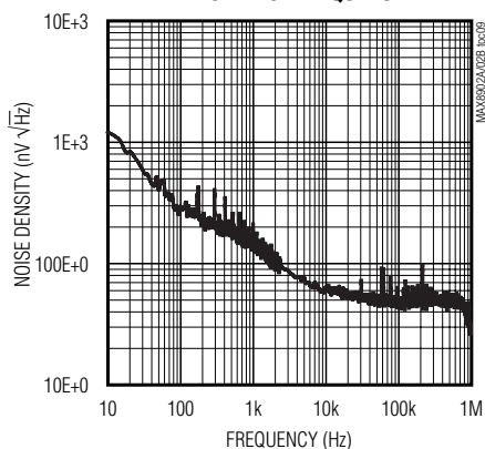
MAX8902A LDO OUTPUT-NOISE SPECTRAL DENSITY vs. FREQUENCY
