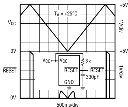
MAX705/MAX707 RESET OUTPUT VOLTAGE vs. SUPPLY VOLTAGE
