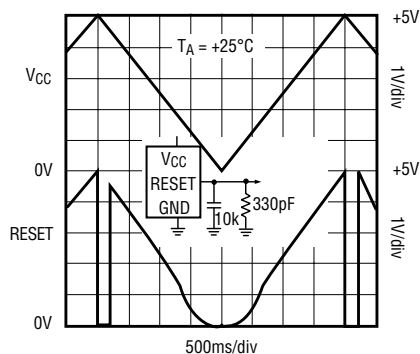
MAX707/MAX708/MAX813L RESET OUTPUT VOLTAGE vs. SUPPLY VOLTAGE
