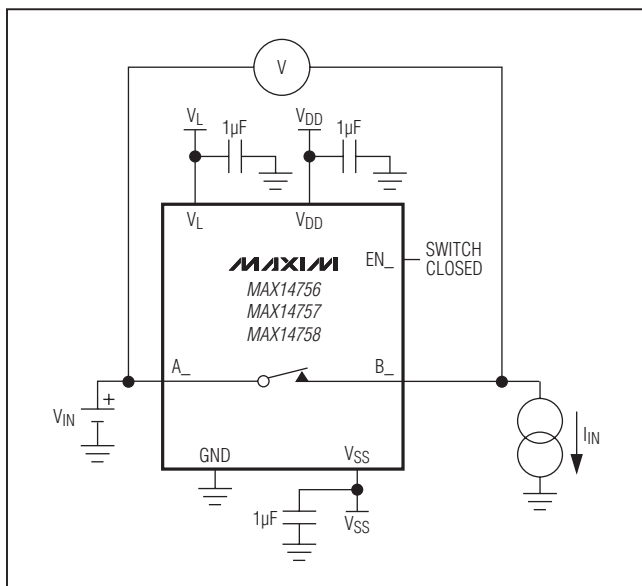
Figure 1. On-Resistance Measurement
