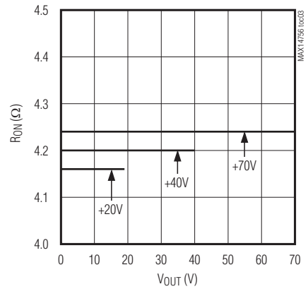
ON-RESISTANCE vs. V_{B-} (SINGLE SUPPLY)
