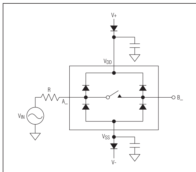
Figure 10. Beyond-the-Rail Application
