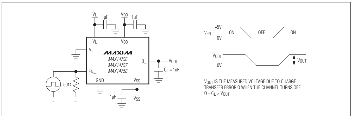
Figure 8. Charge Injection
