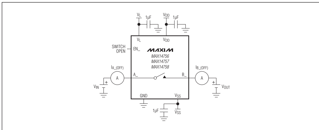
Figure 3. Off-Leakage Current
