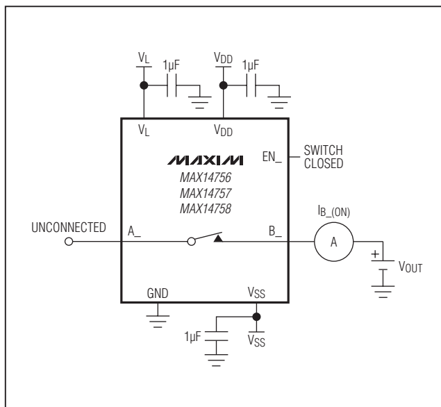
Figure 2. On-Leakage Current
