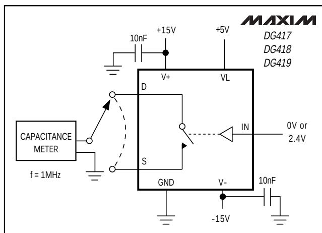
Figure 8. Drain-Source Off-Capacitance
