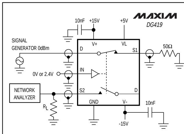
Figure 7. DG419 Crosstalk
