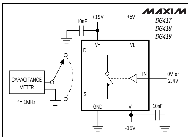
Figure 9. Drain-Source On-Capacitance
