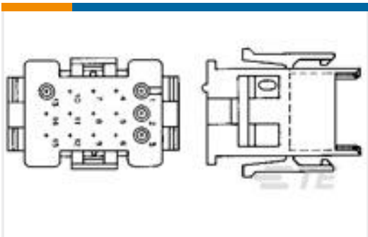
TE Part #1-640512-0 12P MR II CAP HSG V0 RED
