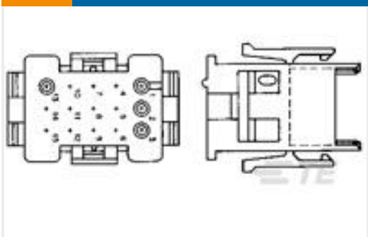
TE Part #1-640509-0 04P MR II CAP HSG V0 RED
