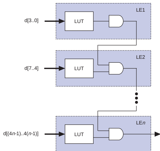
Figure 5. FLEX 8000 Cascade Chain Operation
