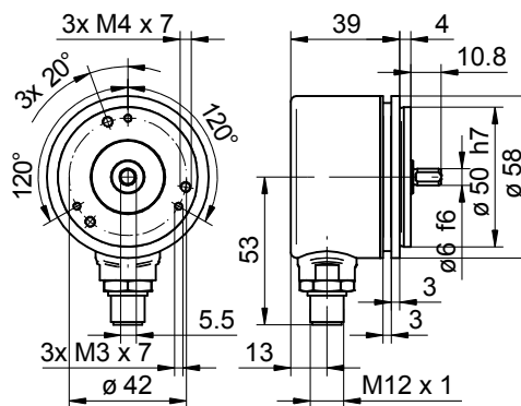
EAM580-SY with flange connector M12
