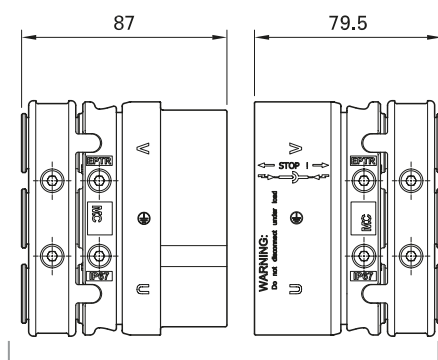
Unmated condition
