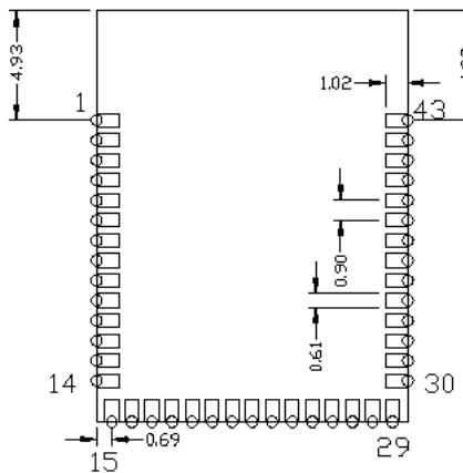
Figure 3. Solder Pad Dimensions
