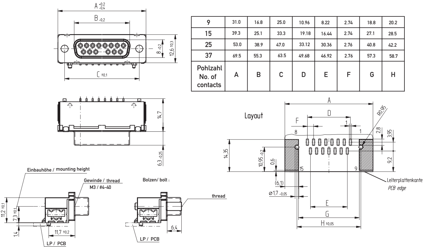
Dimensional Drawing SMT, Assembly Height 7.3 mm
