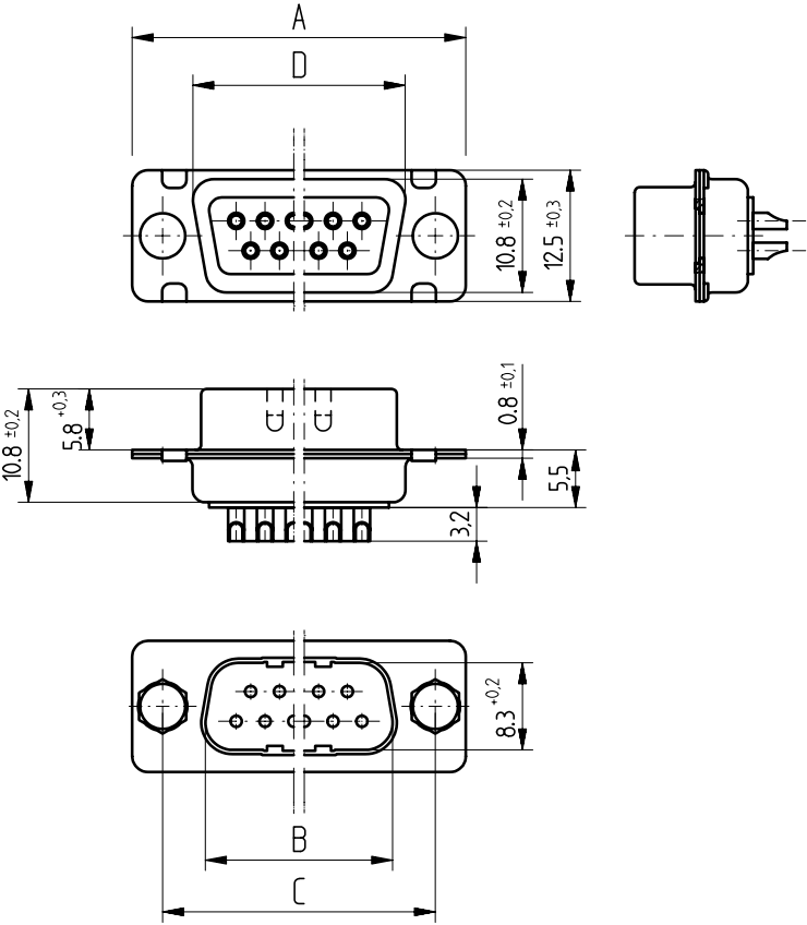
Dimensional Drawing Male Connector
