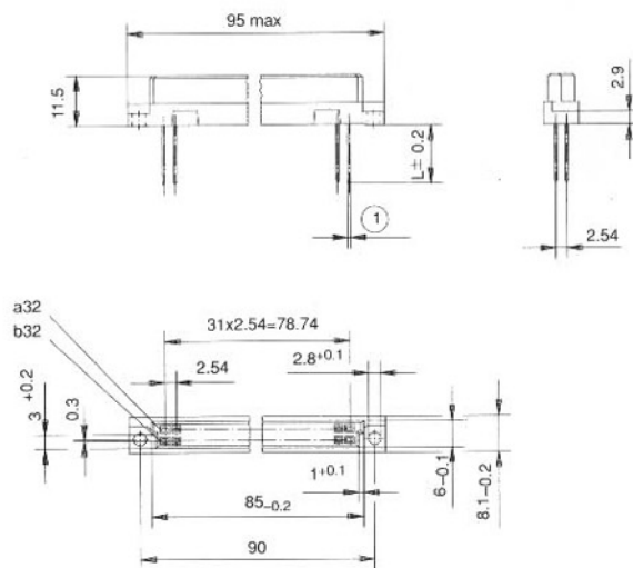
Female connector
