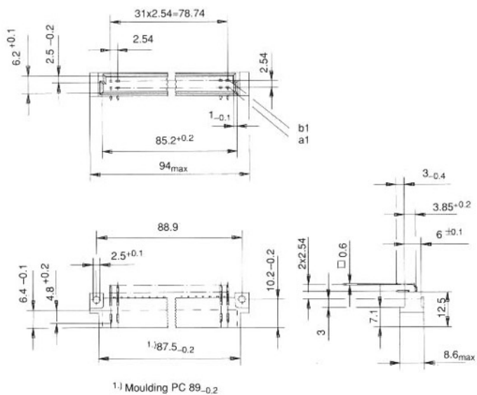
Male connector
