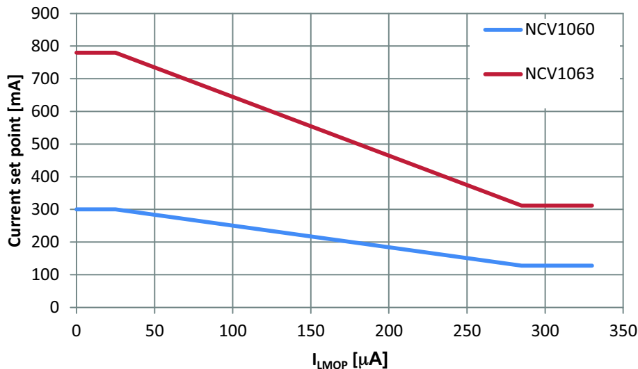
Figure 42. I pk Set-point Dependence on I LMO Current
