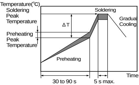
[Standard Conditions for Flow Soldering]
