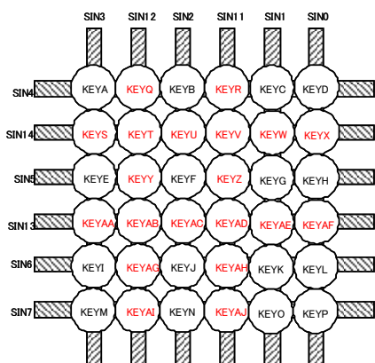
Figure 20. Layout for matrix switch
