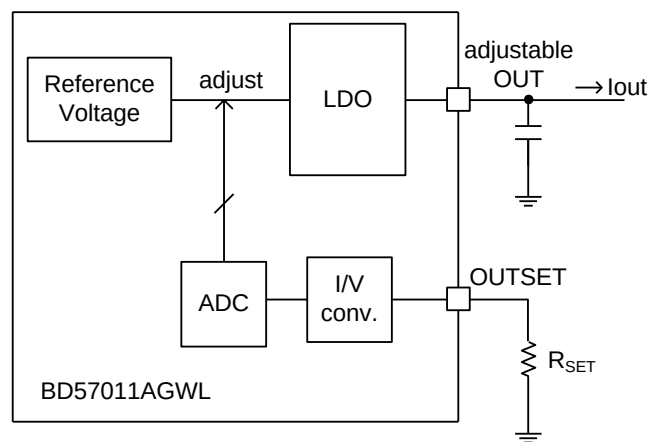
Figure 10. OUTSET circuit
