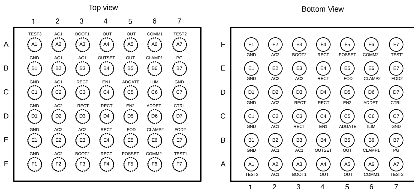
Figure 7. Pin configuration
