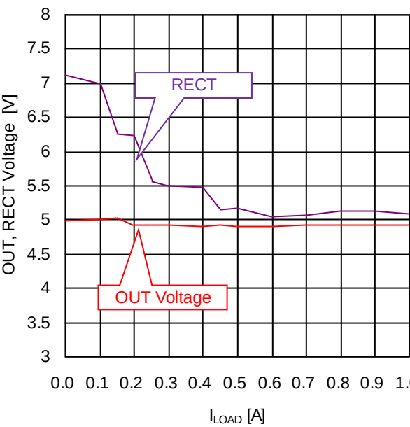
Figure 4. OUT Voltage [V] and RECT Voltage [V] vs. I_{LOAD} [A] ( R_{SET}=27k\ \Omega )
