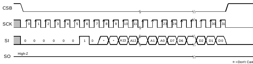
Figure 40. Write command
