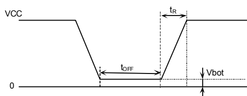
Figure 60. Rise waveform diagram
