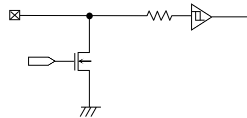
Figure 61. Input / Output Pin Circuit Diagram (SDA)
