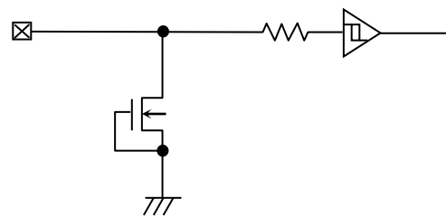
Figure 60. Input Pin Circuit Diagram (SCL)
